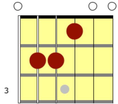
E chord
