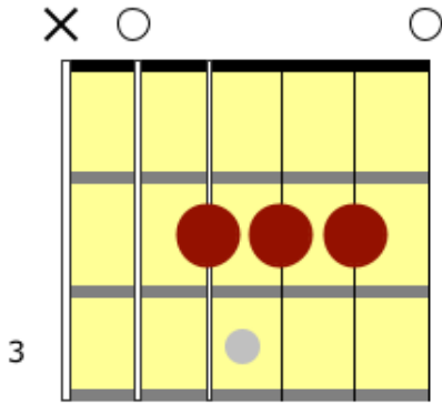
A chord
