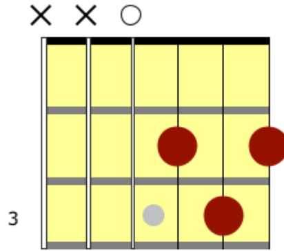
D chord
